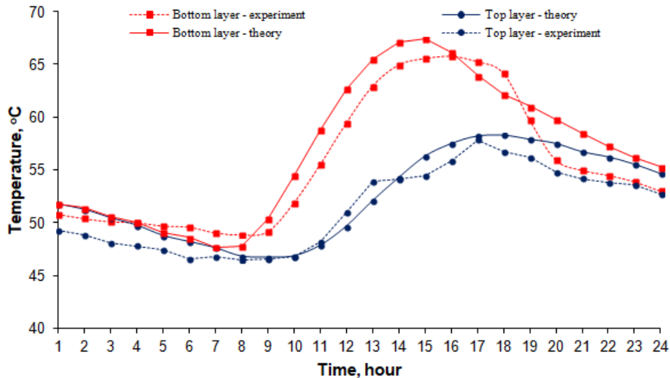
Figure 2. Graph of temperature changes in the upper and lower layers of the heat accumulator capacity of the water tank as a function of time.
