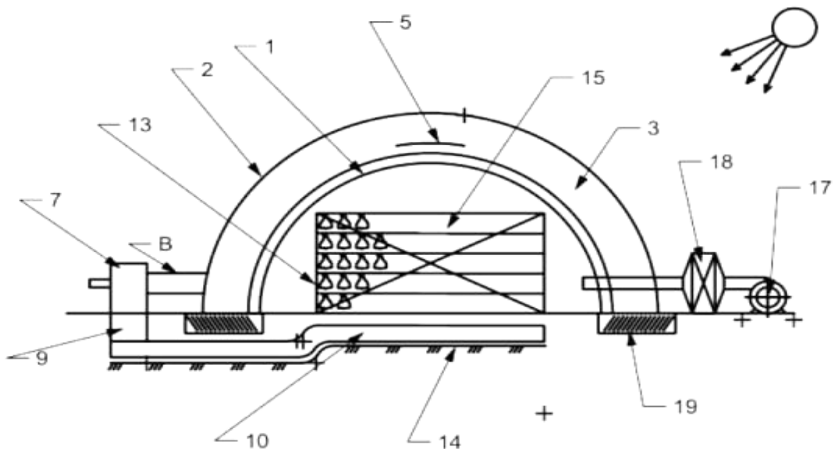
Fig. 2. Cross section of pneumatic dryer
