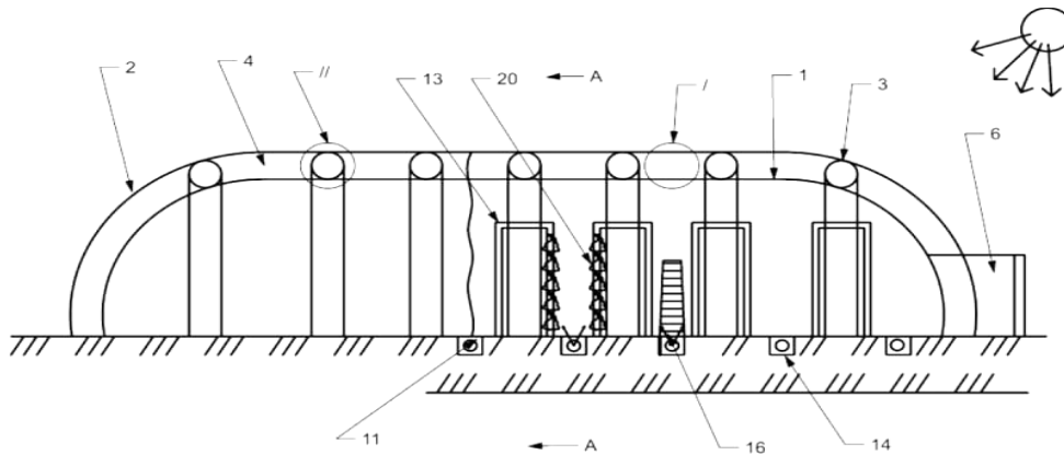
Fig.1. Double-layer pneumatic structure as a solar-radiation drying plant for drying grapes
